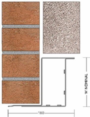
215mm Solid Wall
